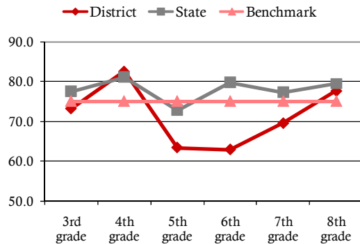
State Math Test Results 1 Proportion Proficient or above
